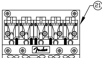
BRIDGE ASSY
