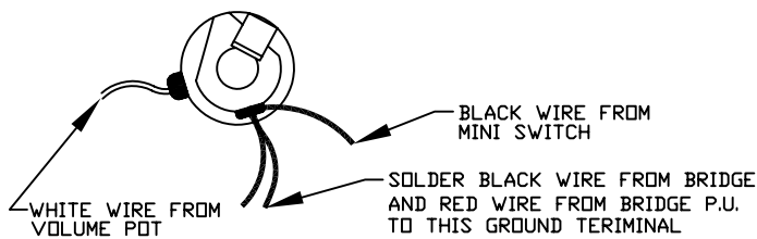
DETAIL "B"
